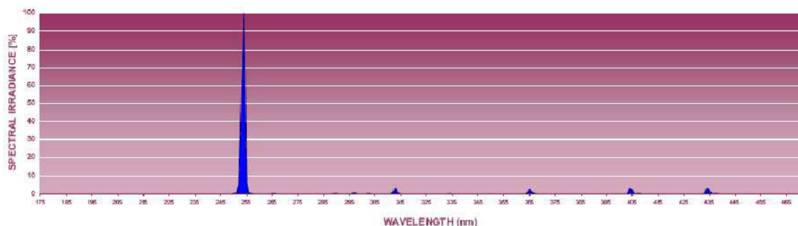
Ozone Free Germicidal Lamp Relative Spectral Energy Distribution
